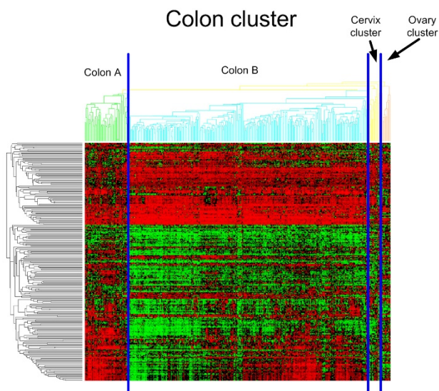
Figure 7 Colon subclustering.
